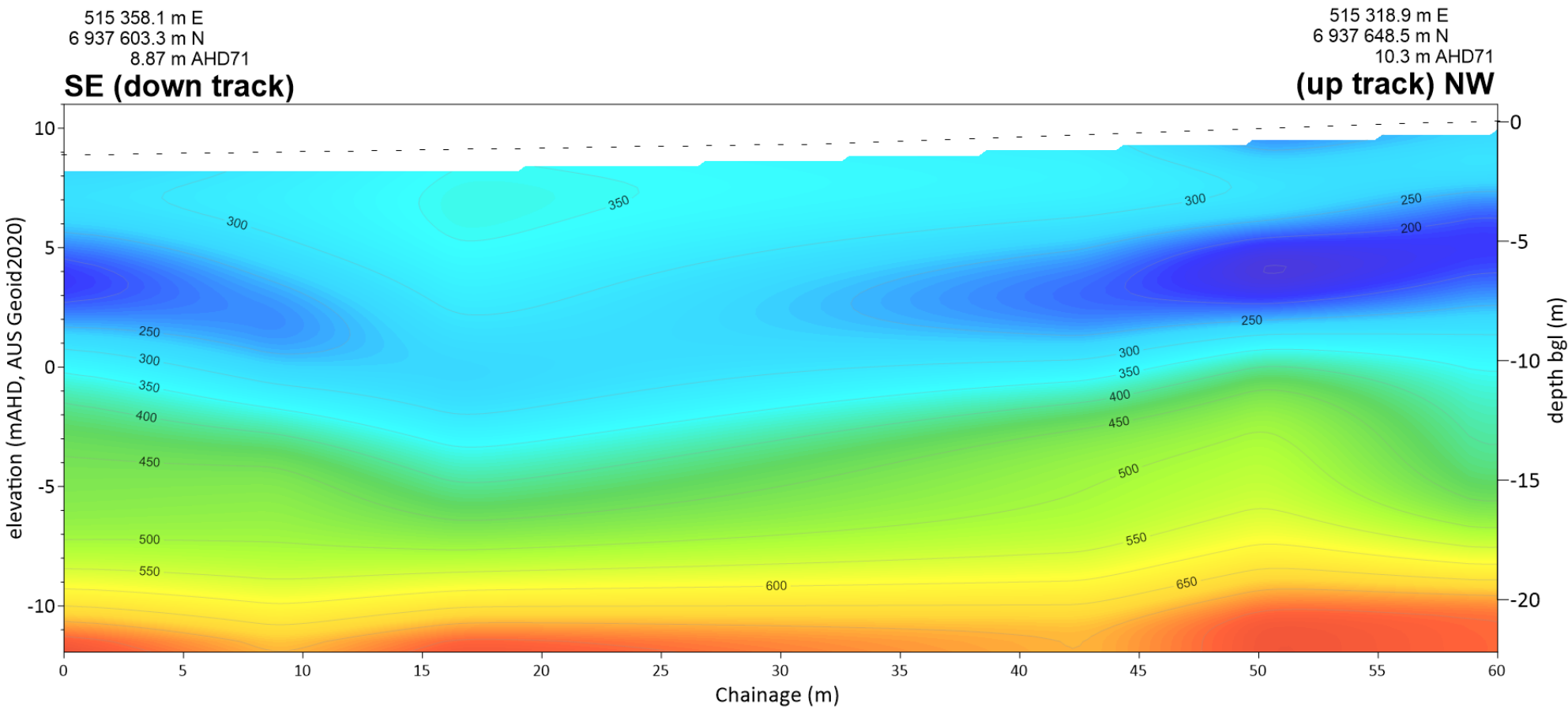
Seismic Line MASW AU-GP 165-4
